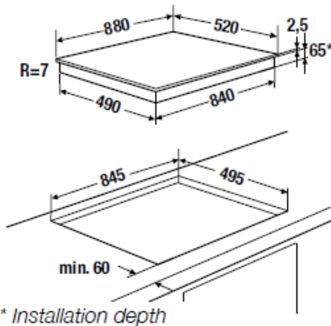
Top mount installation
