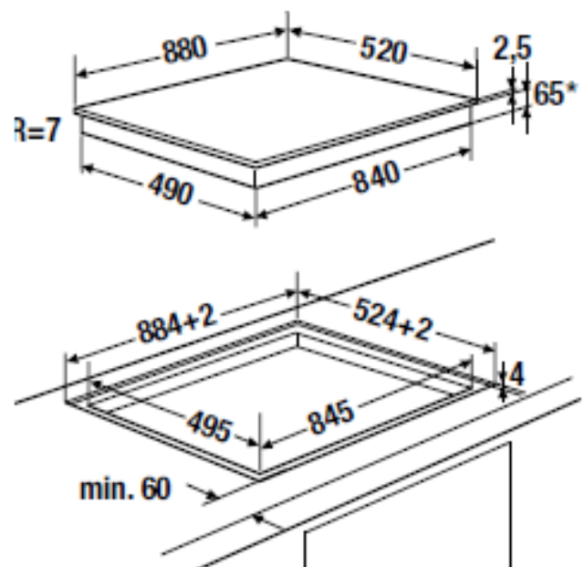
Flush installation
